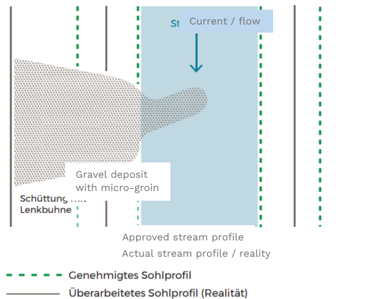
Figure 15: Gravel micro-groin in top view as a measure to restructure the overly wide, overly deep profile 12
