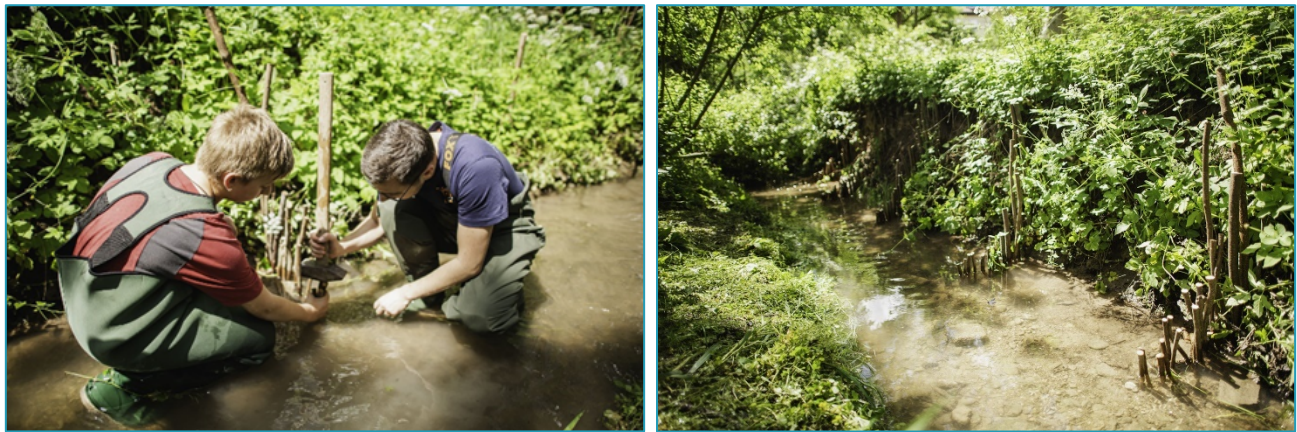
Figure 8: Installation of the sticks with the hammer (left) at low water level, arrangement of the sticks (sloping towards the middle of the stream); photos: © Peter Runkewitz
