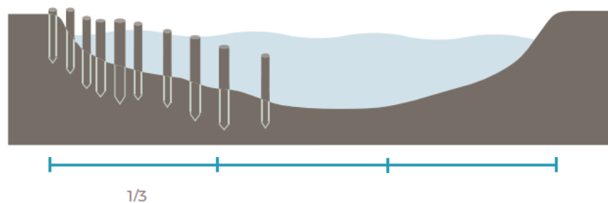
Figure 9: Added wood structure at mean water level in the stream cross-section. © Luise Schumann
