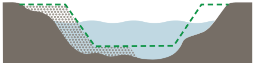
Figure 12: Gravel micro-groin in cross profile
